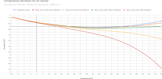
Temperature deviation for air sensor
